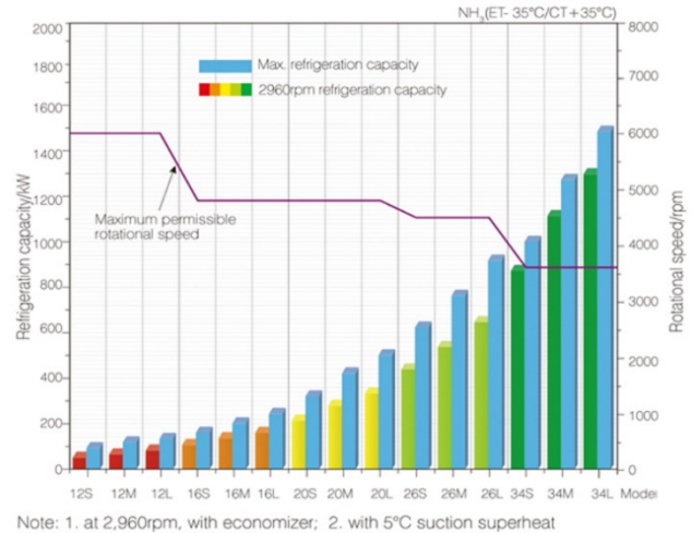
Refrigeration Capacity of SRMP1V Open-type Single-stage Inverter Screw
